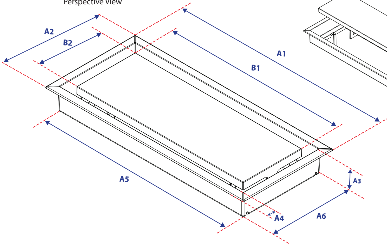
Component Dimensions
