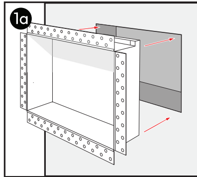
Dry fit body into vent opening
